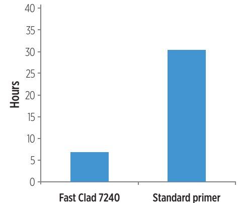
Comparison graph: Drying time to handle @ 5°C
